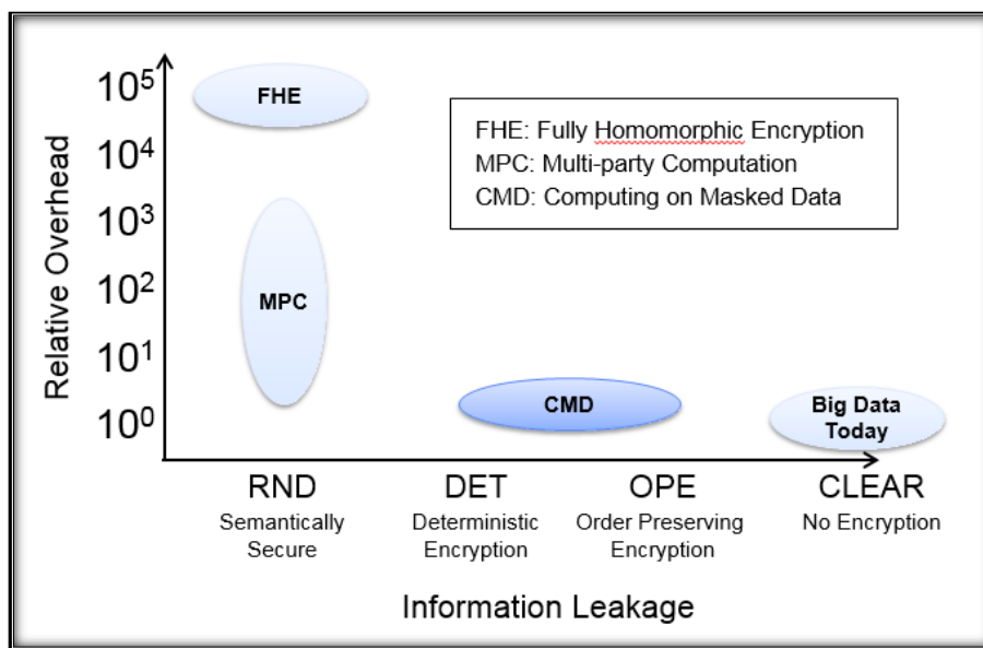
Figure 6. Computational overhead of different cryptographic techniques. Cryptographic protection adds significant computational cost. For example, the most effective protection schemes (FHE and MPC) require massive computation and communication overhead respectively. Yet medical and bioinformatics computations must add cybersecurity protections to protect privacy of patients and meet HIPAA regulations. The cryptographic overhead alone could push workstation codes into the exascale regime. Courtesy of Dr Patrick Dreher (Massachusetts Institute of Technology and North Carolina State University), Dr. Chris Hill (Massachusetts Institute of Technology), Dr. John Quackenbush (Harvard School of Public Health).
