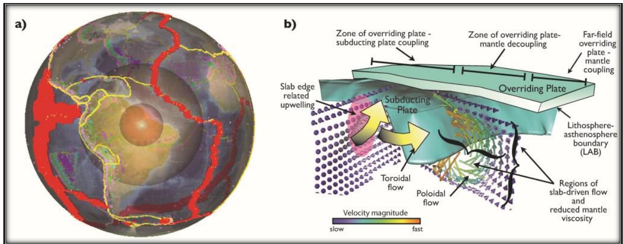
Figure 2. Multiscale global and regional tectonics. Large-scale computational resources will allow geophysicists to model and simulate plate tectonics at higher-resolutions and increased physical accuracy. (a) Observational constraints on the nature of tectonic plates, overlain on the major structural boundaries within the Earth. (b) Results from a high-resolution 3D regional model of a single plate boundary show small-scale convection. Convection on Earth contains small-scale, highly non-linear processes shown in (b) embedded within the larger-scale, whole mantle convection that occurs in (a). Image courtesy of M. A. Jadamec (University of Houston); modified from Jadamec, J. Geodynamics v. 100:51-70, 2016.
