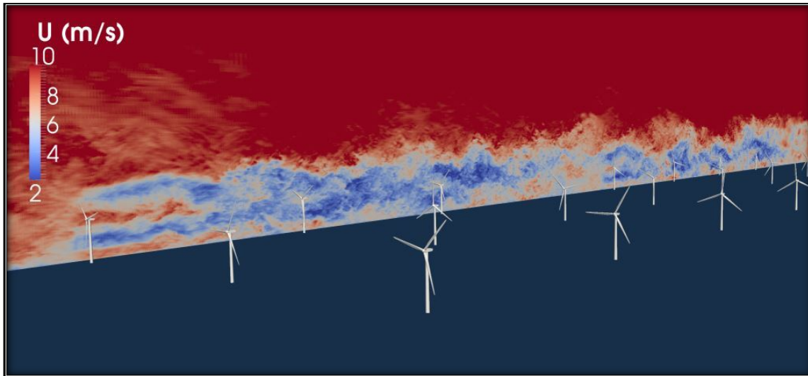
Figure 3. Systems level modeling of a wind farm. Energy production from individual wind turbines depends on plant-level dynamics. Predictive, physics-based, high-fidelity modeling of wind farms at the full-plant level is critical to accurately predict and optimize wind farm performance. Exascale resources will allow for dramatic improvements in wind farm systems modeling and predictability and facilitate wide-scale development of cost-competitive wind energy facilities. Courtesy of Matt Churchfield, National Renewable Energy Laboratory, Golden CO.
