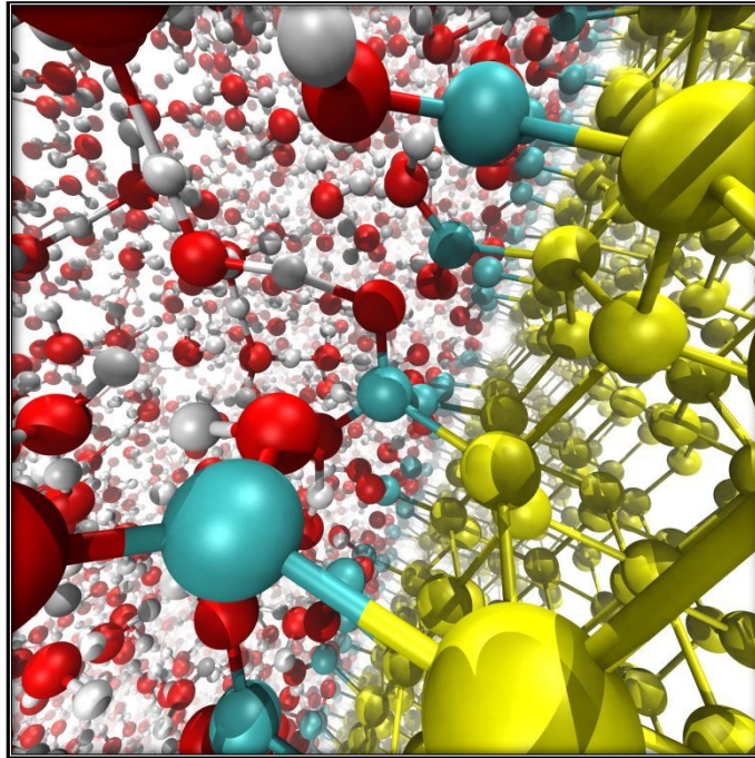
Figure 1. Si-COOH/water interface. Exascale resources will allow unprecedented large-scale first-principle simulations on the atomic scale. With a greater number of atoms and longer time scales, exascale resources will substantially bolster scientists' ability to predict and engineer the properties and functions of materials. Image courtesy Giulia Galli and Marco Govoni (Argonne National Laboratory and University of Chicago).
